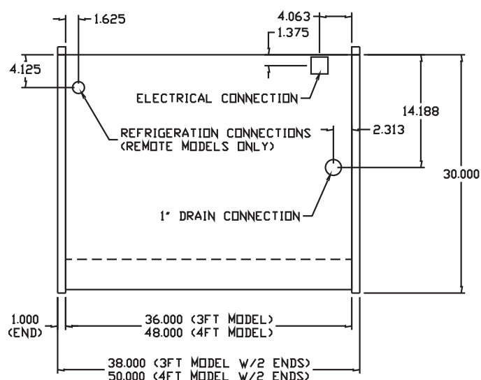
Plan Views
